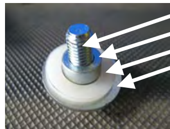
M10 x 30 bolt Spacer bush M16 nylon washer Large M10 washer
