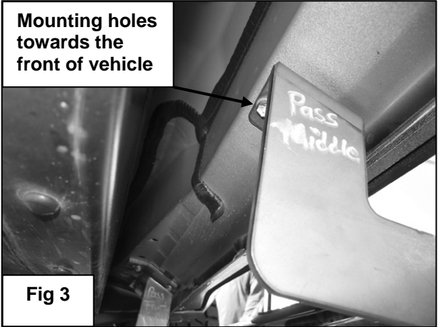
Center Passenger Side Mounting Bracket
